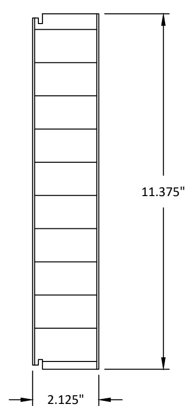
103 2-1/4" SLAB, 11-3/8" CLAD BOTTOM RAIL WOOD
