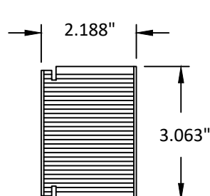
97 2-1/4" SLAB, 3-1/16" CLAD RAIL WOOD
