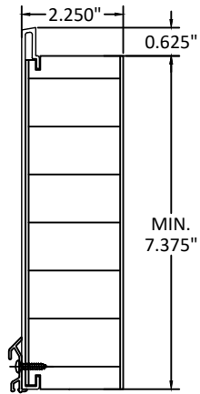
8" BOTTOM RAIL
