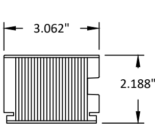
85 2-1/4" SLAB, 3-1/16" CLAD STILE WOOD
