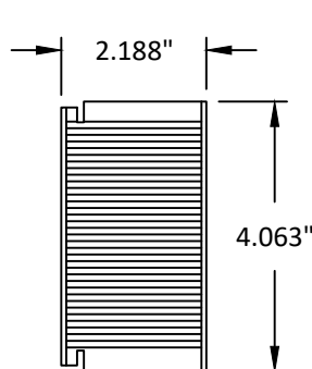
96 2-1/4" SLAB, 4-1/16" CLAD RAIL WOOD
