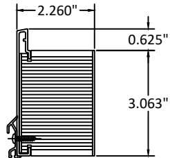
3-11/16" BOTTOM RAIL
