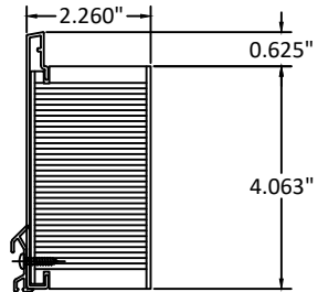
4-11/16" BOTTOM RAIL
