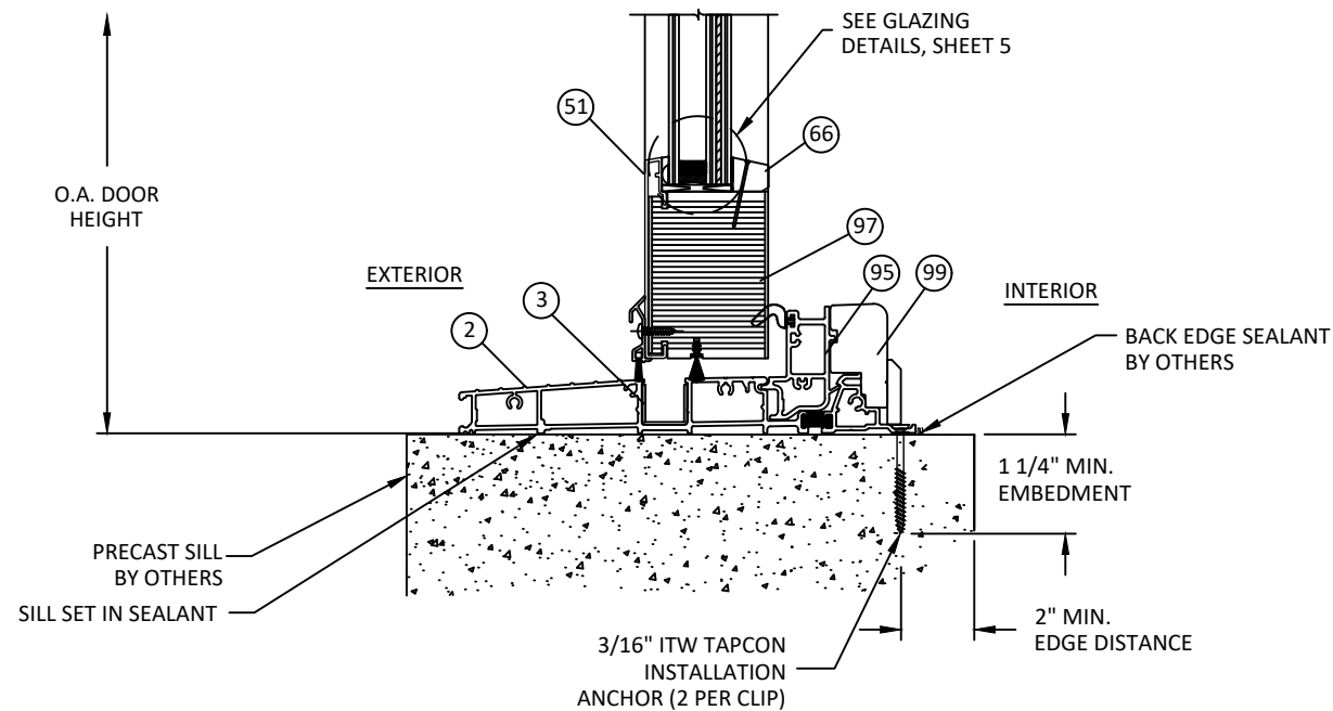
B 4 VERTICAL SECTION SILL - PRECAST CONCRETE HIGH PERFORMANCE SILL
