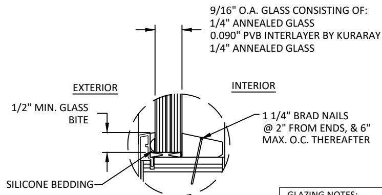
GLAZING DETAIL 2
